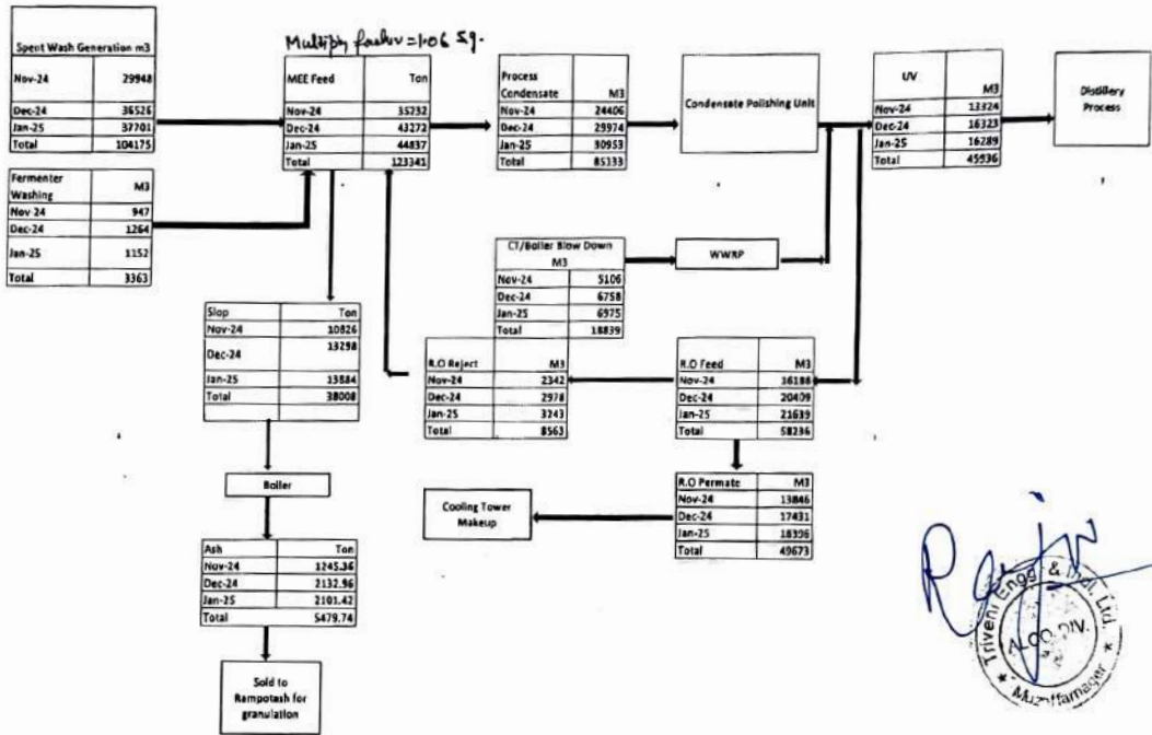
Spent Wash Management Scheme Flow Diagram(ZLD) Triveni Engineering & Industries LTD, Alco Chemicals Complex, Muzaffarnagar
